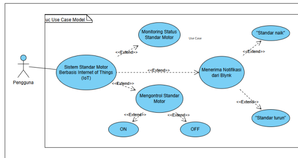
Gambar 8. Use Case Diagram
