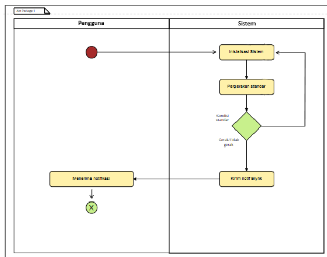
Gambar 9. Activity Diagram
