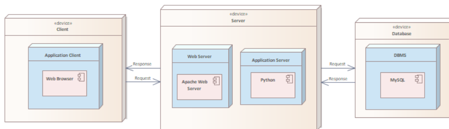
Gambar 11 Deployment diagram
