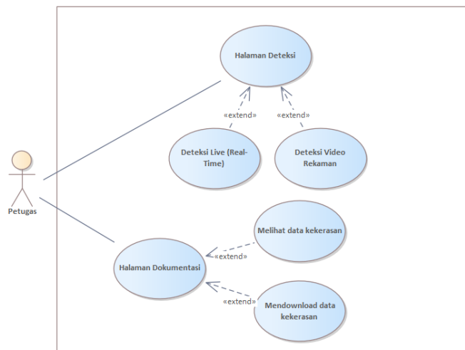
Gambar 10 Usecase Diagram
