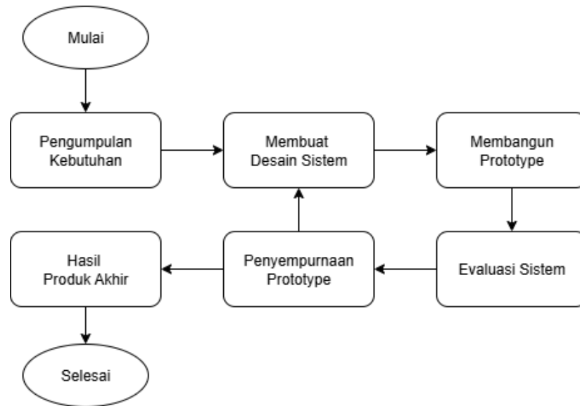
Gambar 4 Model Prosedural
