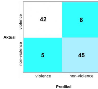
Gambar 13 Confusion Matrix
